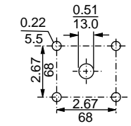
Four-Hole 90 x 90 Mounting Dimensions [8]
