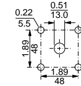
Four-Hole 60 x 60 Mounting Dimensions [8]
