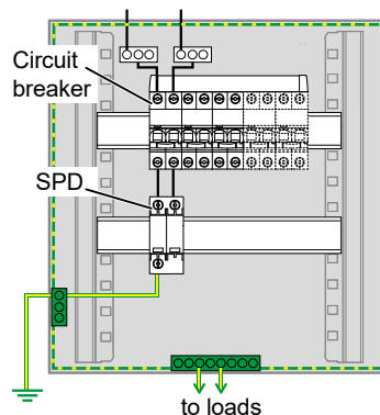
How to connect a SPD in a metallic enclosure
