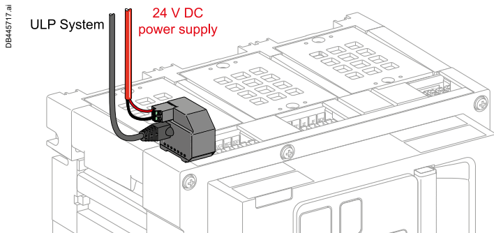
ULP Port Module for MasterPacT MTZ1/MTZ2/MTZ3 Fixed
