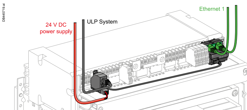
ULP Port module for MasterPacT MTZ2/MTZ3 Drawout with EIFE
