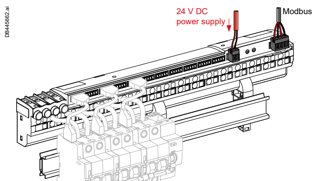
I/O Smart Link with Linergy FM Installation
