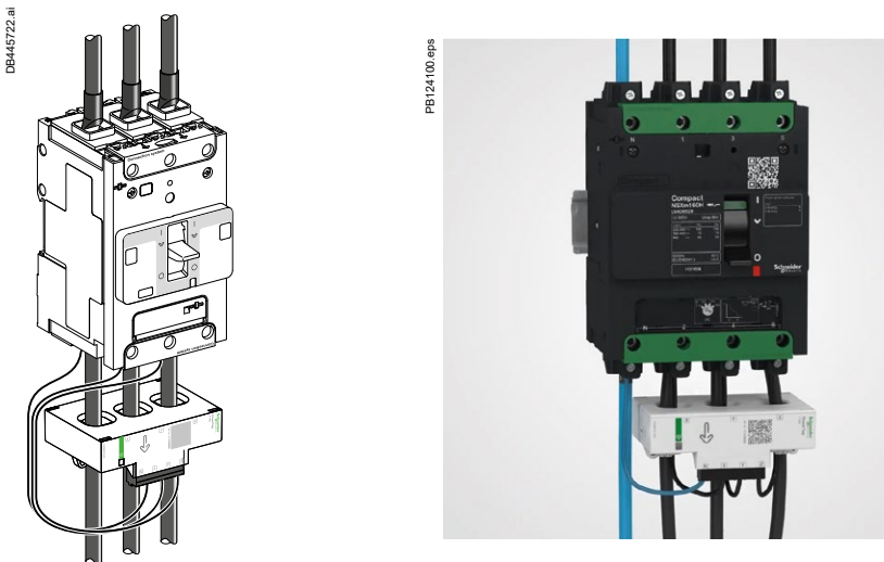
PowerTag Energy F160 mounted downstream of a ComPacT NSXm circuit breaker (3P left, 3P+N right)
