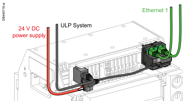
ULP Port Module for MasterPacT MTZ1 Drawout with EIFE
