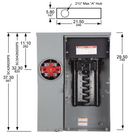
Surface Mount type "SC-" (Ring Type, no bypass)
