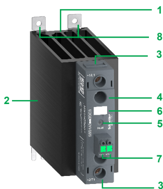
SSD1 single-phase solid state DIN rail contactor with pluggable spring input, 45(mm)/1.77(in)
