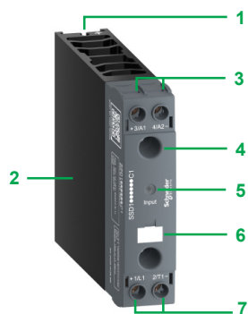
SSD1 single-phase solid state DIN rail relay, 22.5(mm)/0.89(in)
