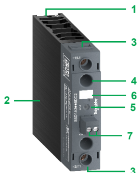
SSD1 single-phase solid state DIN rail contactor with pluggable screw input, 22.5(mm)/0.89(in)
