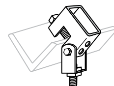
U563 Beam Clamp with Swing Hanger ¾" set screw included. Rod sizes: ¾" Design load 540 lbs.
