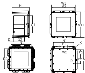
JBX12124 - JBX16160
