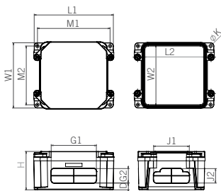
JBX442 - JBX666
