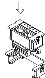
Pass & Seymour ACTIVATE Bezel and Communication Jack
