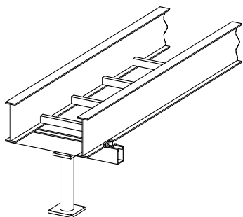
Figure 3-25 Elevated Strut-Type Support
