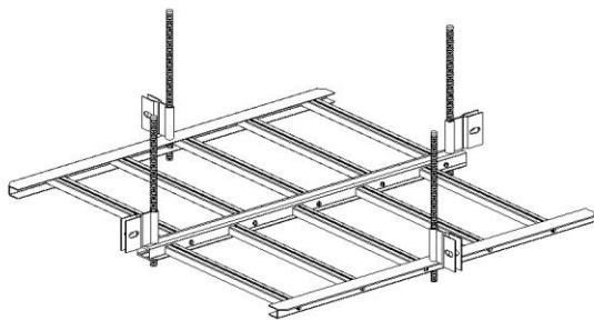
Figure 3-52 Horizontal Hub
