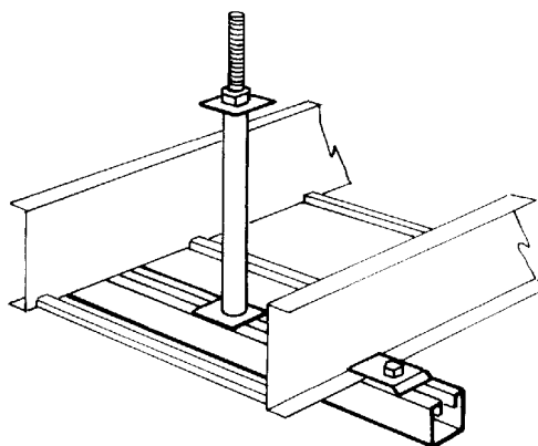
Figure 3-14 Center Hanger Support
