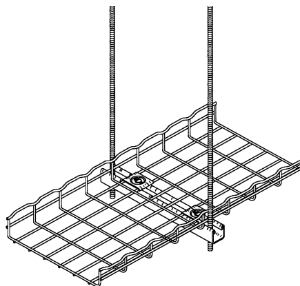
Figure 3-7 Hold Downs
