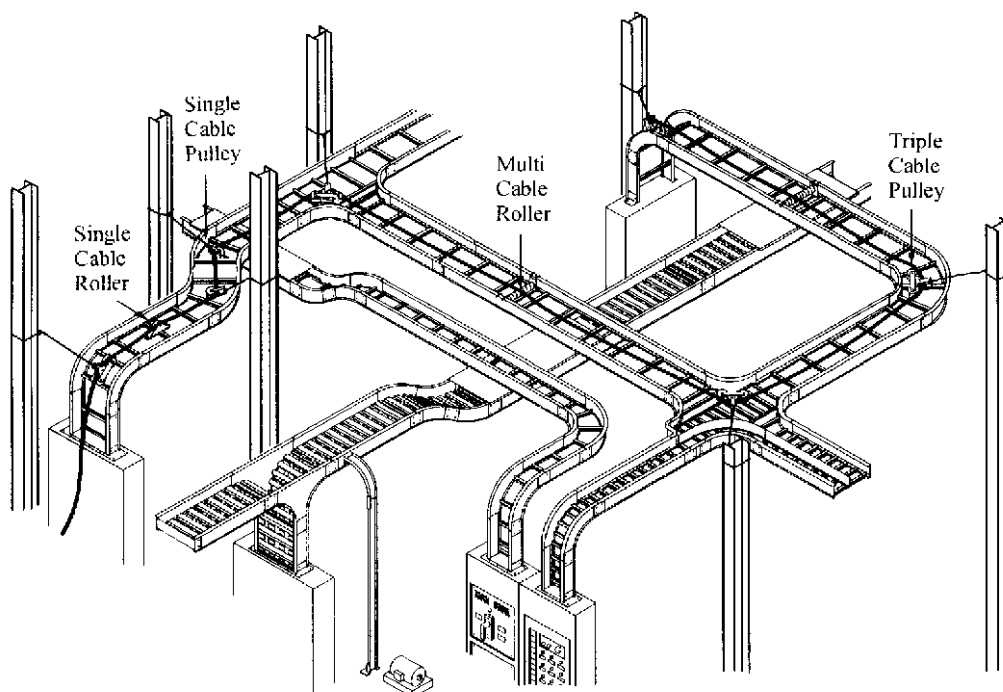
Figure 4-1 Cable Installation
