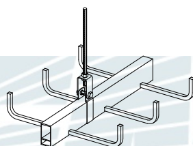
Figure 3-19 Clevis Hanger
