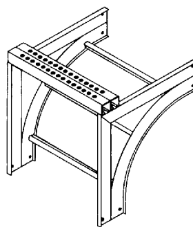
Figure 3-62 Vertical Cable Support
