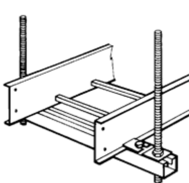
Figure 3-3 Strut Support
