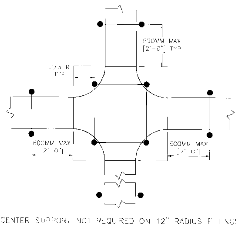
Figure 3-57 Horizontal Cross
