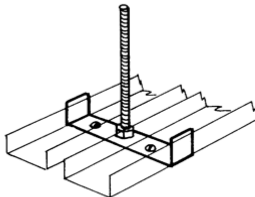
Figure 3-16 Double Channel Hanger
