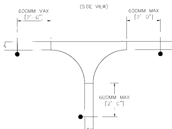
Figure 3-60 Vertical Tee (Side View)
