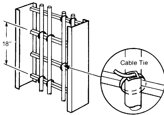
Figure 4-7 Cable Ties—Vertical Application
