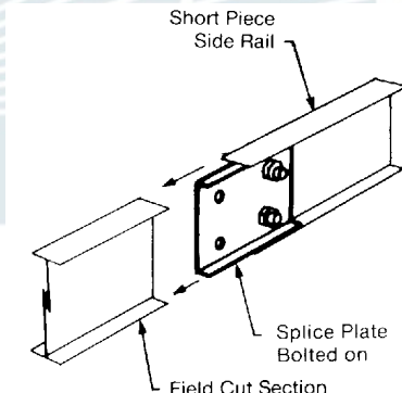
Figure 3-74 Drilling with Punched Side Rail
