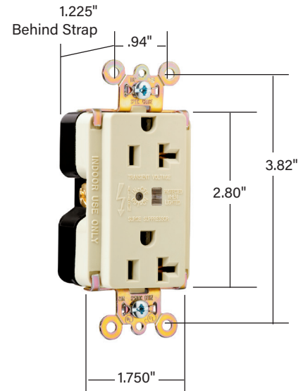
Dimensions for 15 & 20 Amp
