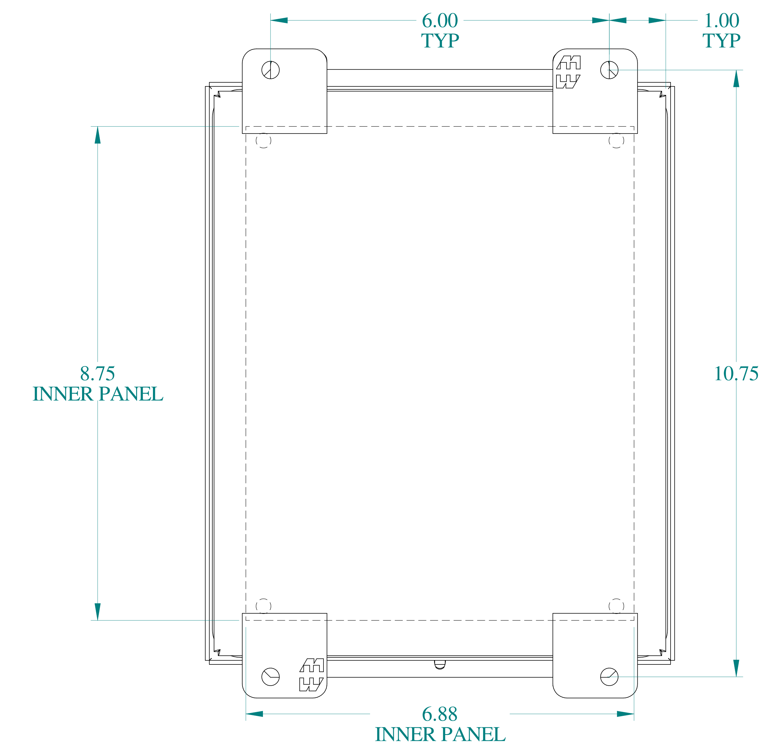
BACK VIEW
