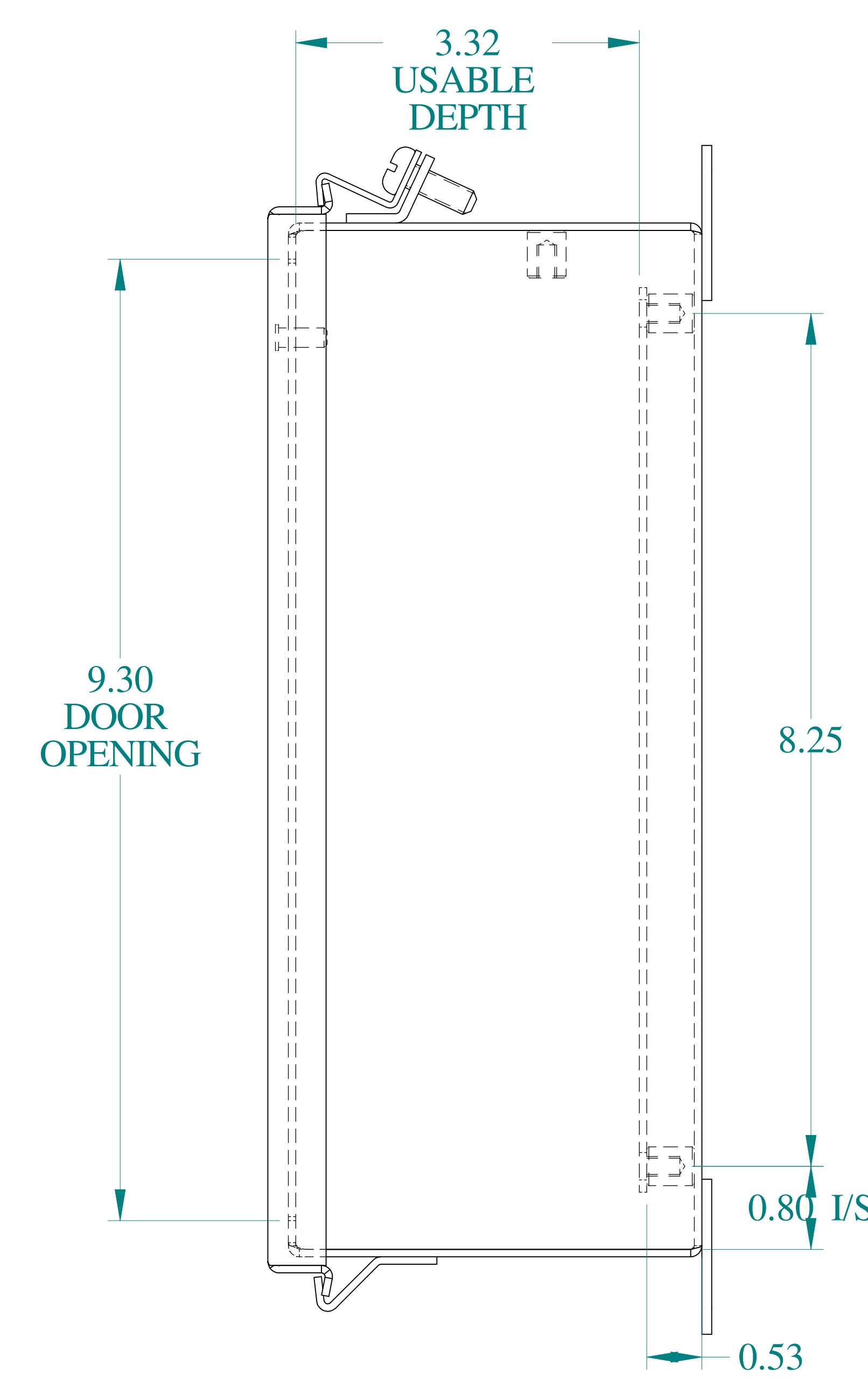
SIDE VIEW
