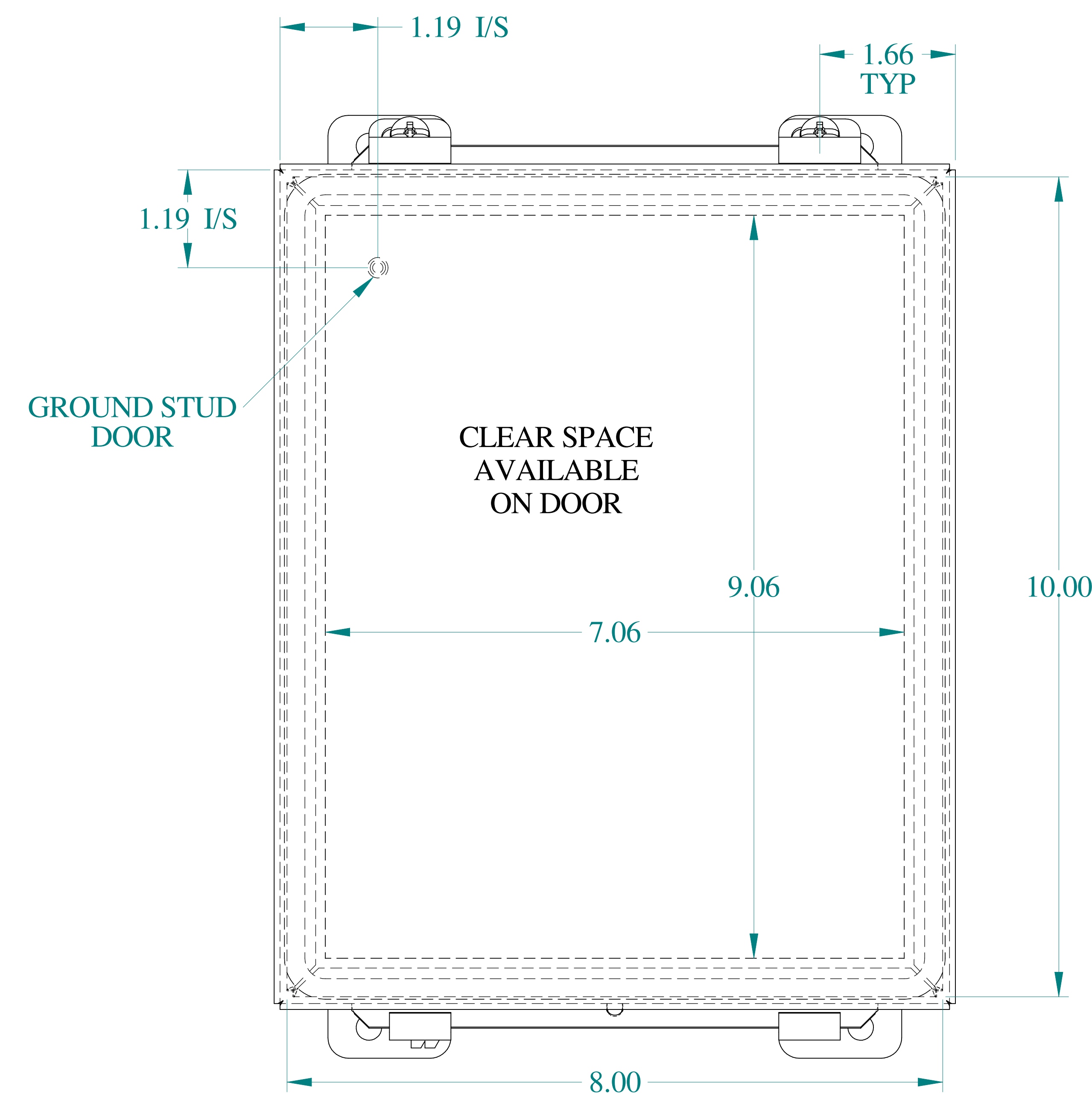
FRONT VIEW
