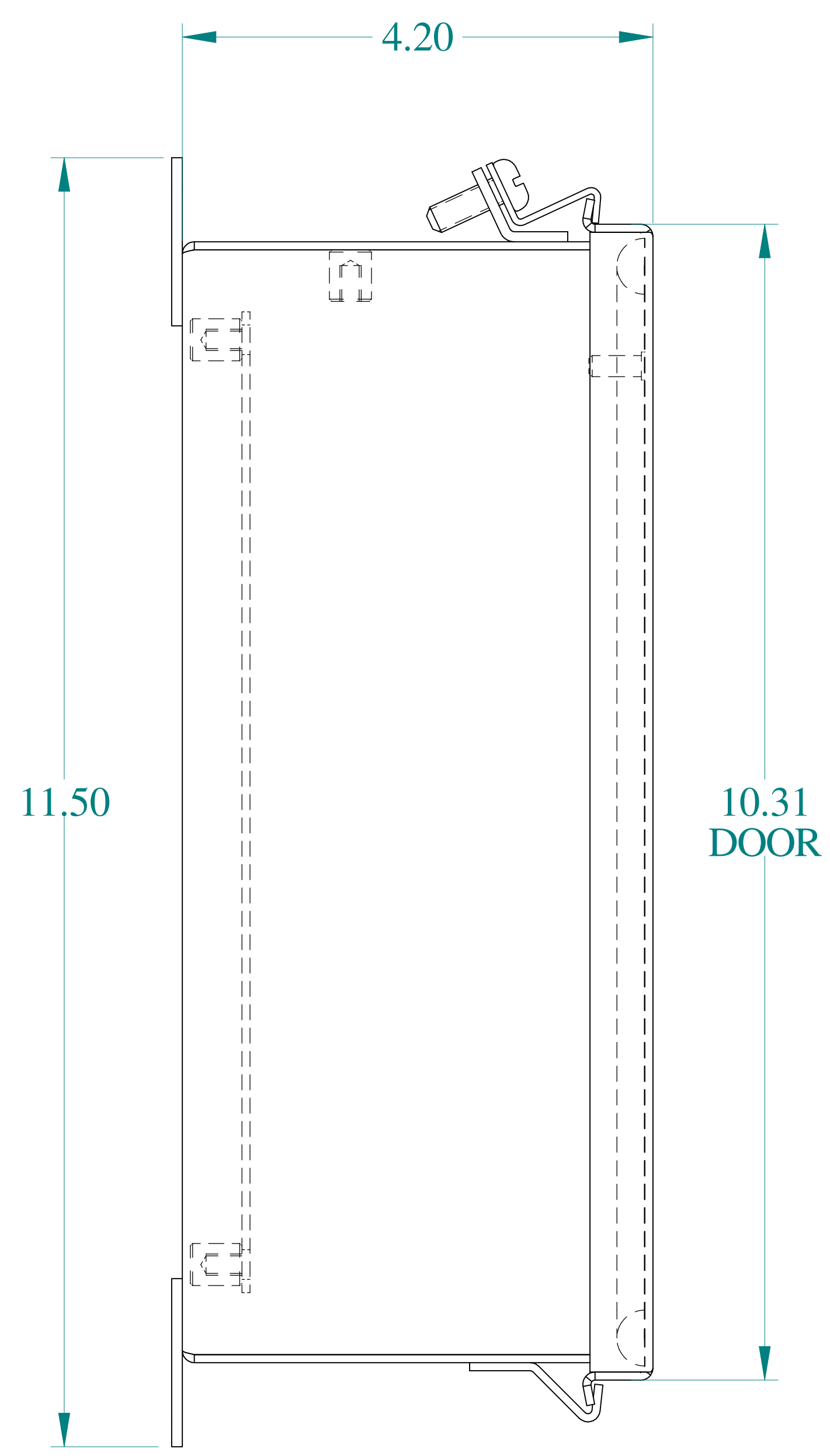
SIDE VIEW
