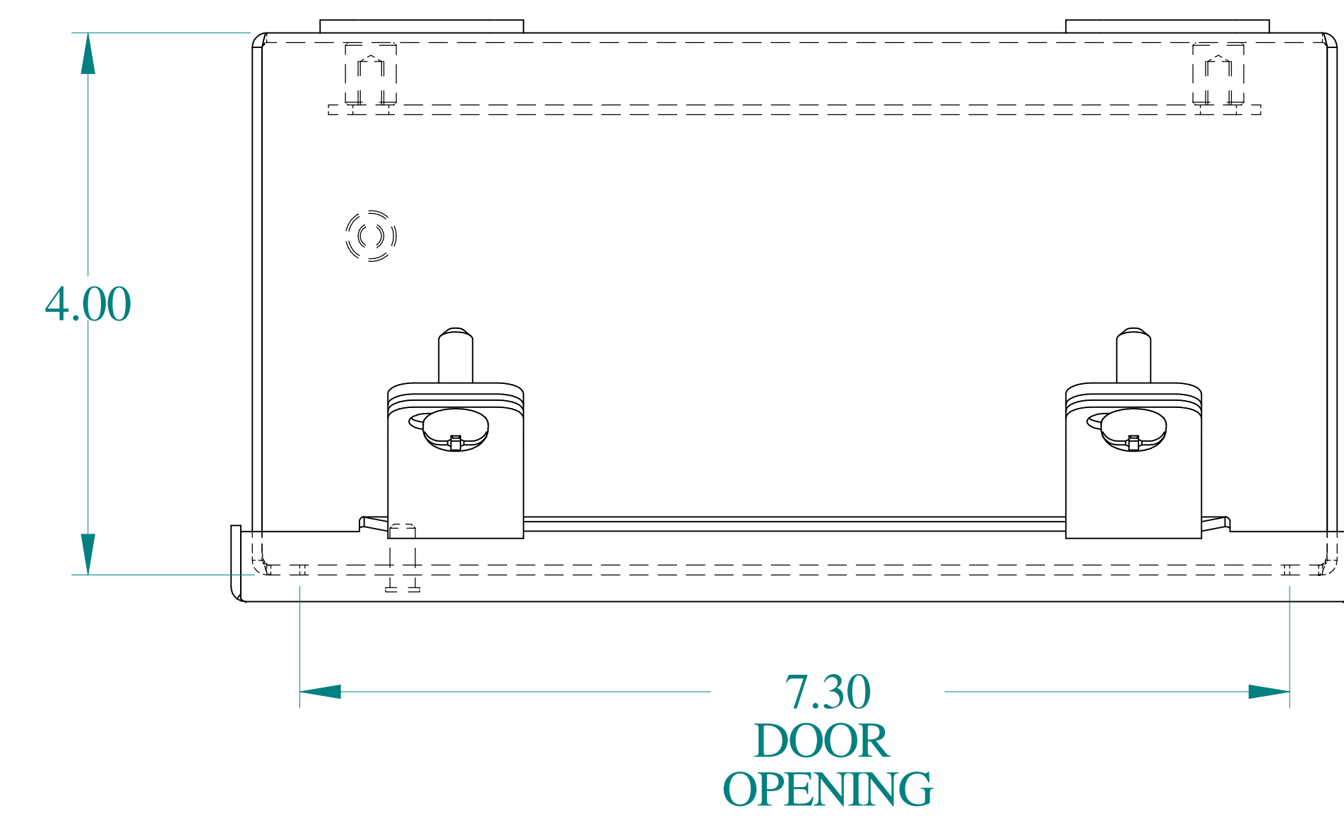
TOP VIEW
